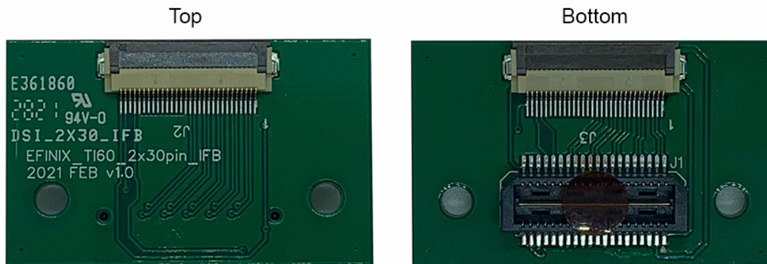
Figure 1: Dual MIPI to DSI Converter Daughter Card
