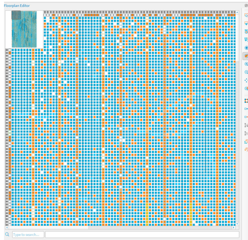
Figure 6 32-Bit RISC-V Processor Design Floorplan
