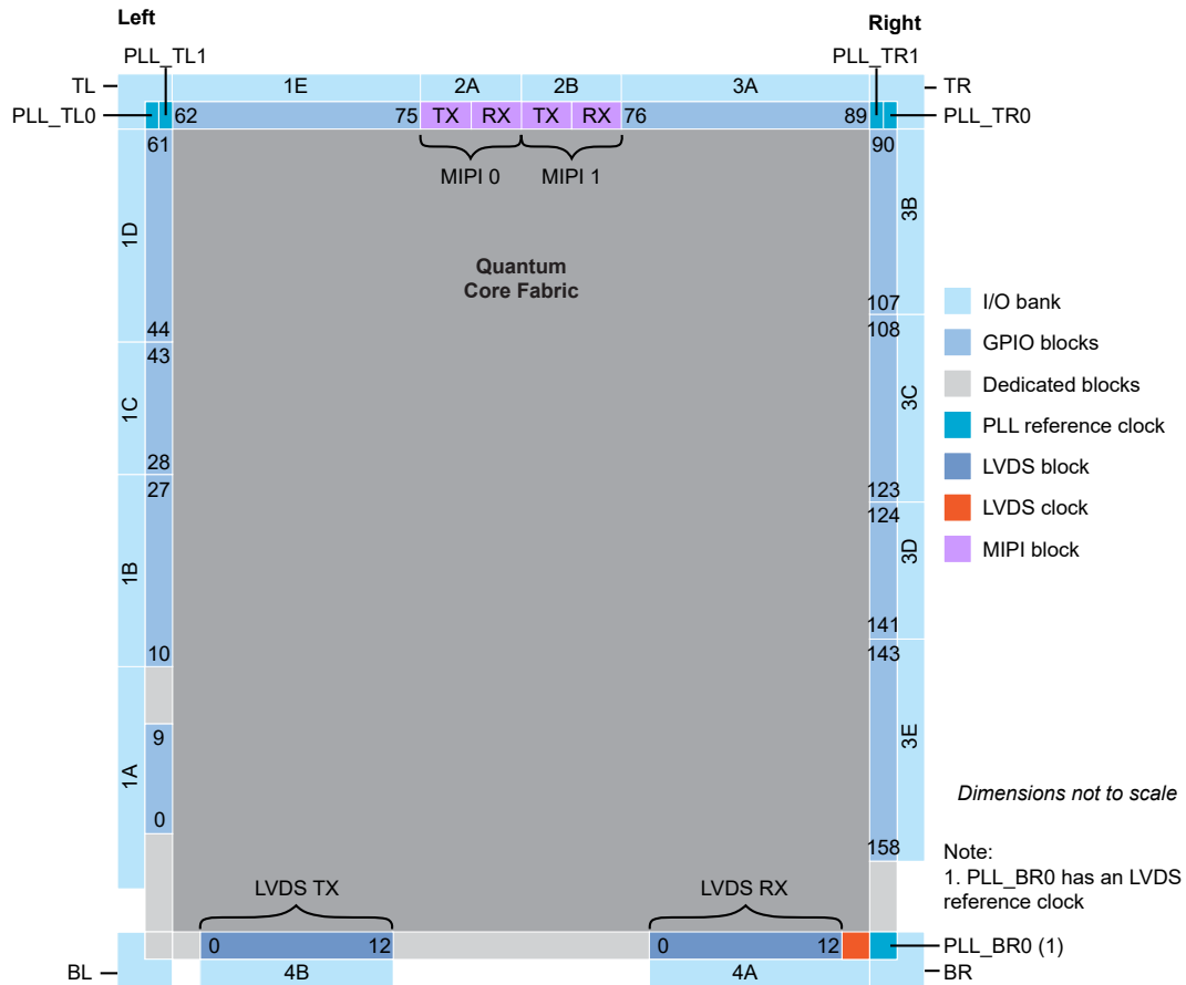
Figure 40: Floorplan Diagram for FPGAs in F169 Packages (with MIPI)
