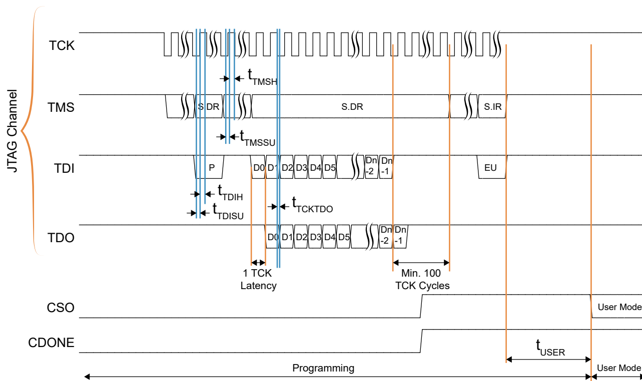
Figure 37: JTAG Programming Waveform (F324 and F400 Packages)
