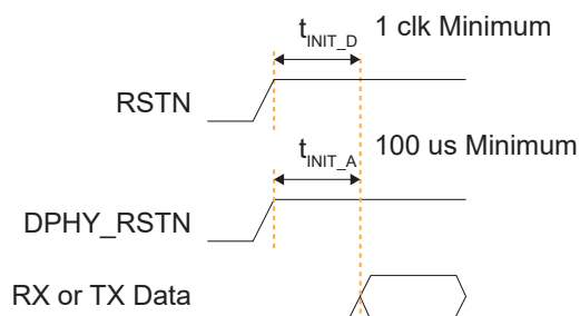
Figure 33: DPHY_RSTN and RSTN Timing Diagram
