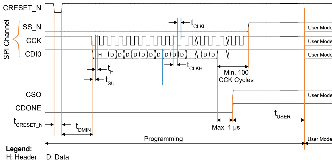
Figure 35: SPI Passive Mode (x1) Timing Sequence
