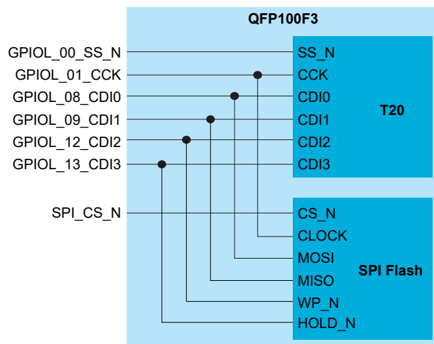
Figure 27: Connections between FPGA and SPI Flash Device inside the Package
