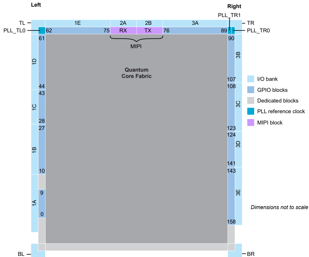
Figure 38: Floorplan Diagram for FPGAs in W80 Packages (with MIPI)
