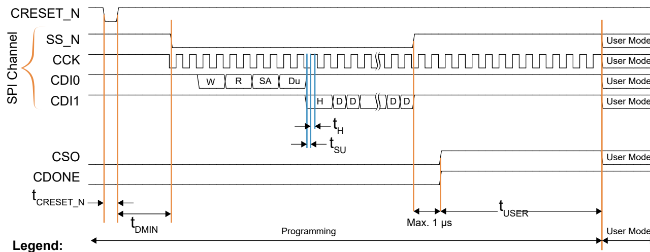
Figure 34: SPI Active Mode (x1) Timing Sequence
