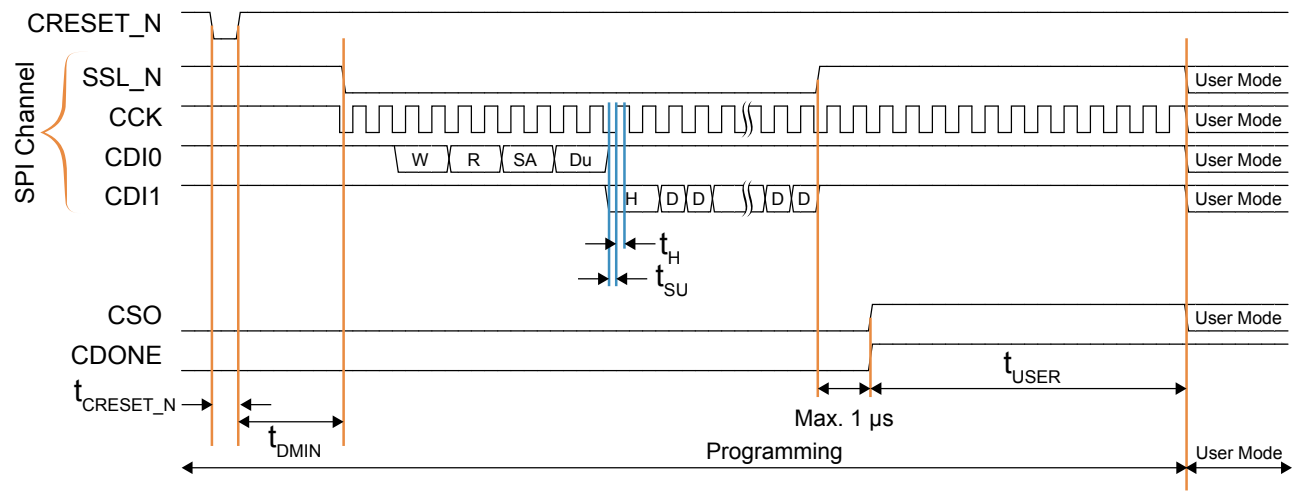
Figure 50: SPI Active (x1) Timing Sequence
