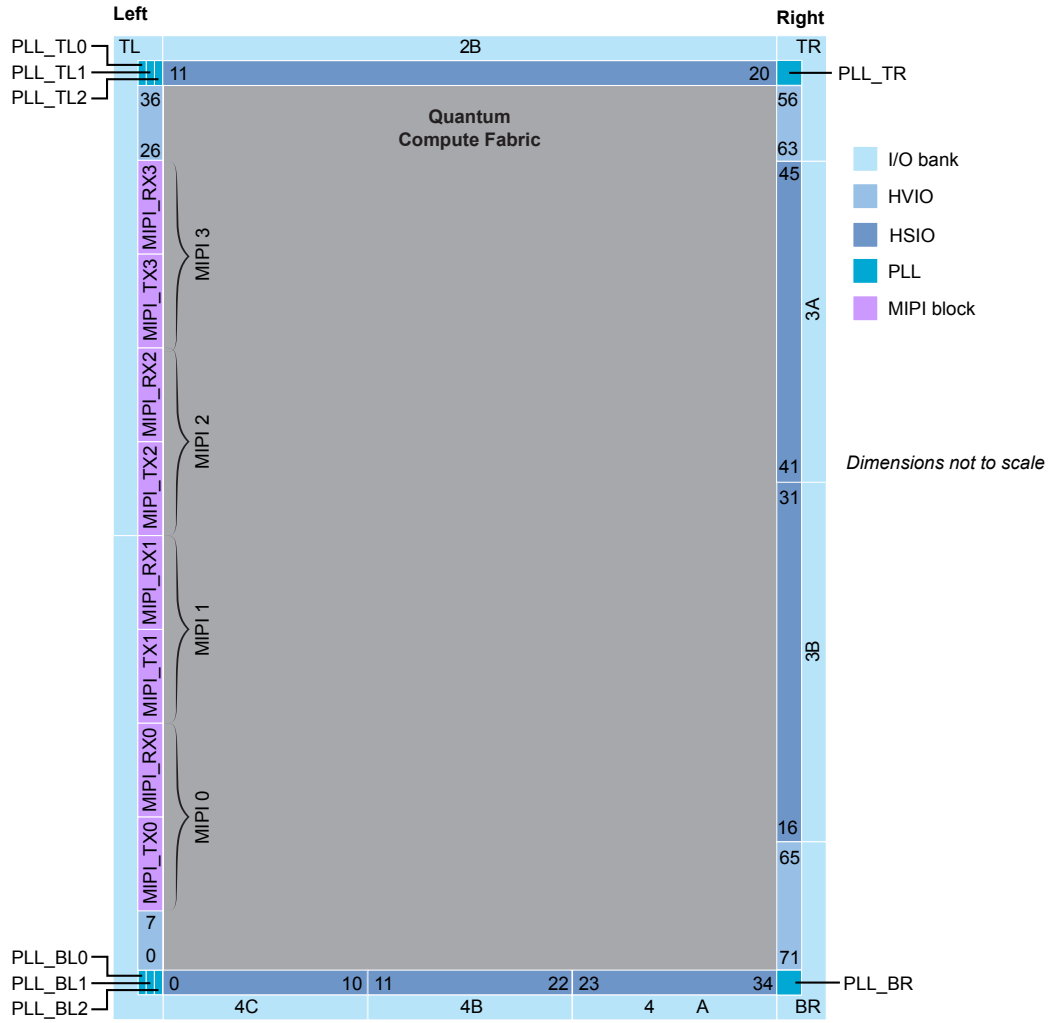
Figure 54: Floorplan Diagram for L484 Packages
