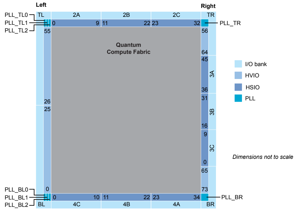
Figure 53: Floorplan Diagram for G400 Packages
