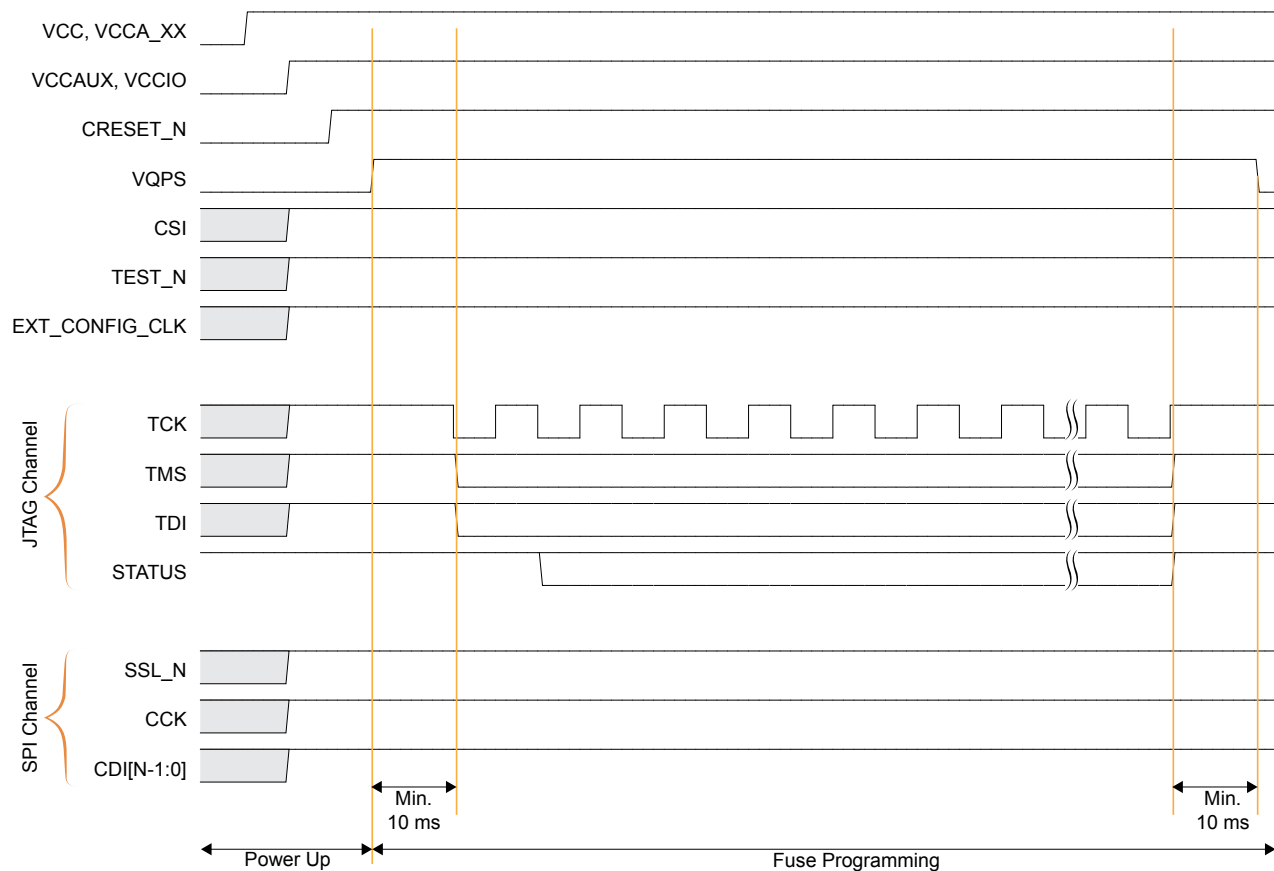
Figure 45: Fuse Programming Waveform
