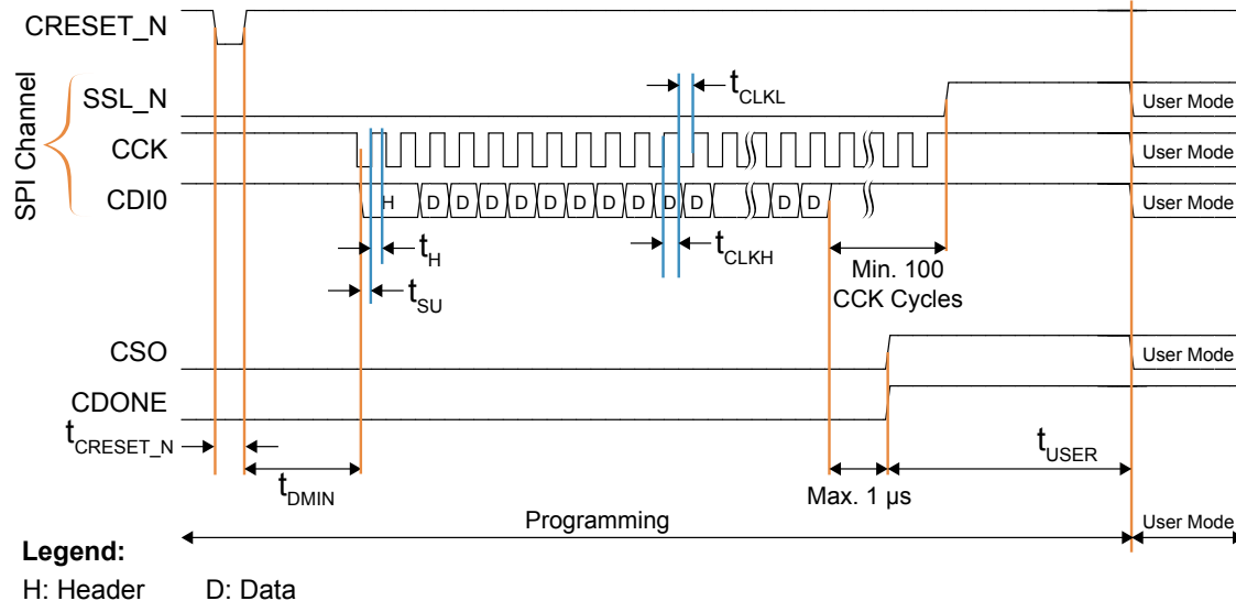
Figure 53: SPI Passive Mode (x1, Mode 3) Timing Sequence
