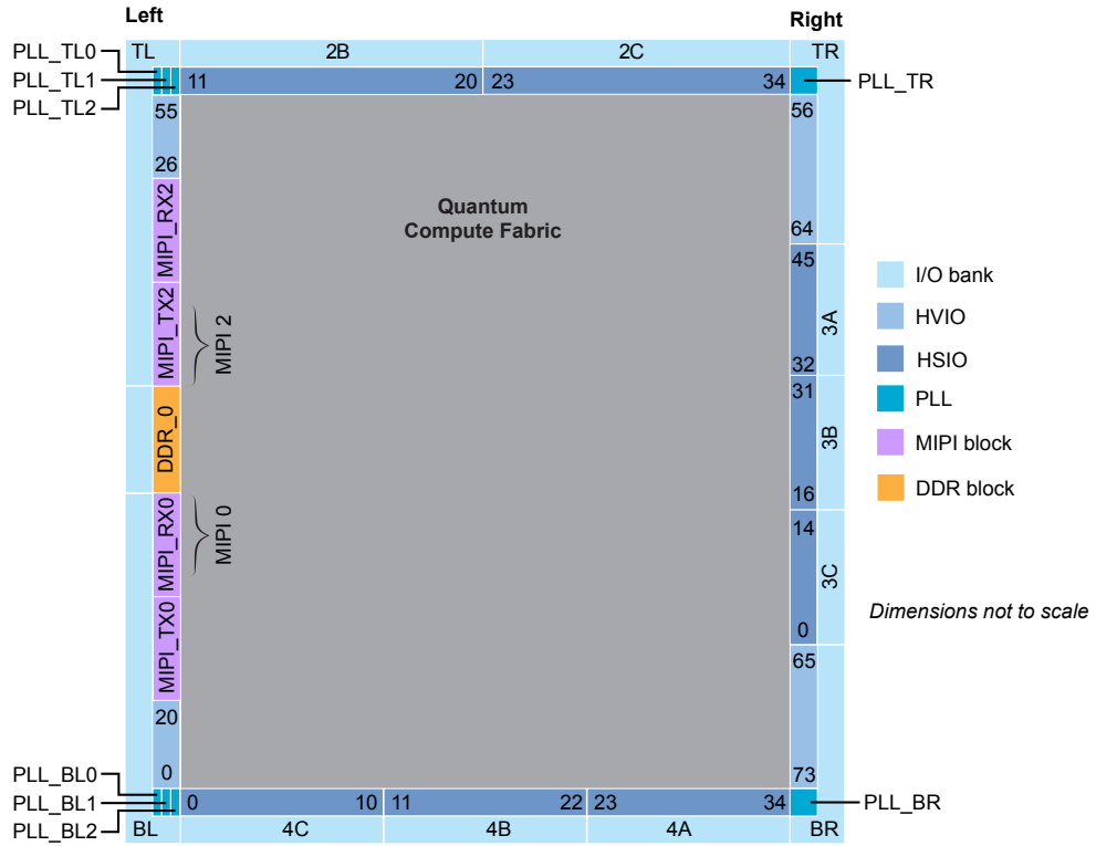
Figure 58: Floorplan Diagram for J484D1 Packages
