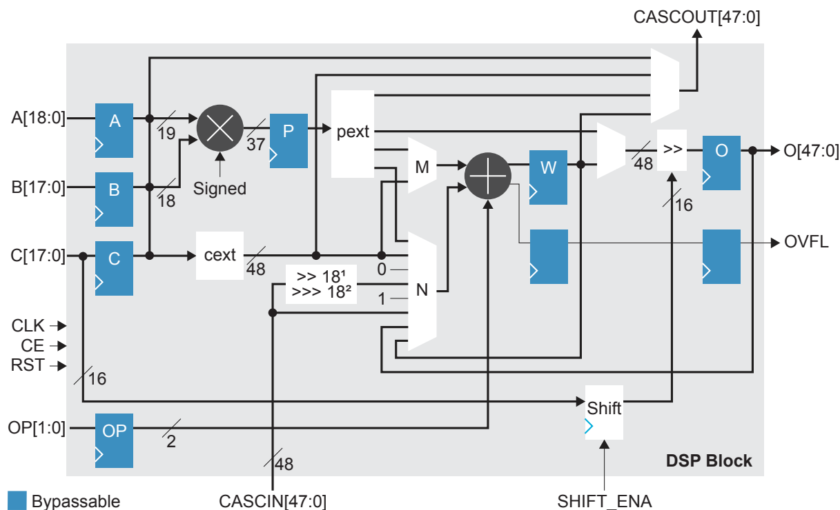
Figure 5: DSP Block Diagram
