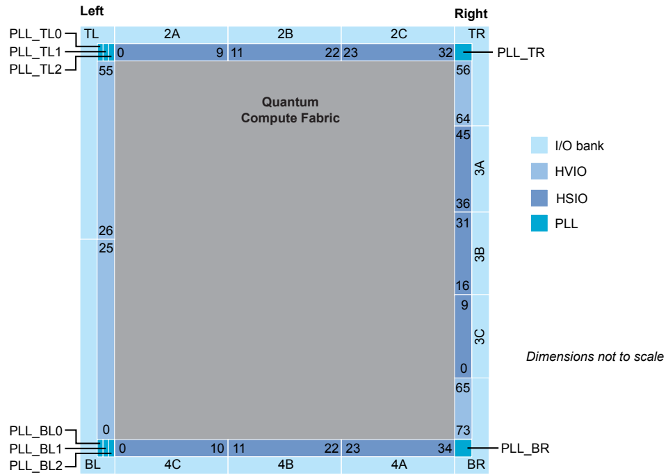
Figure 55: Floorplan Diagram for G400 Packages
