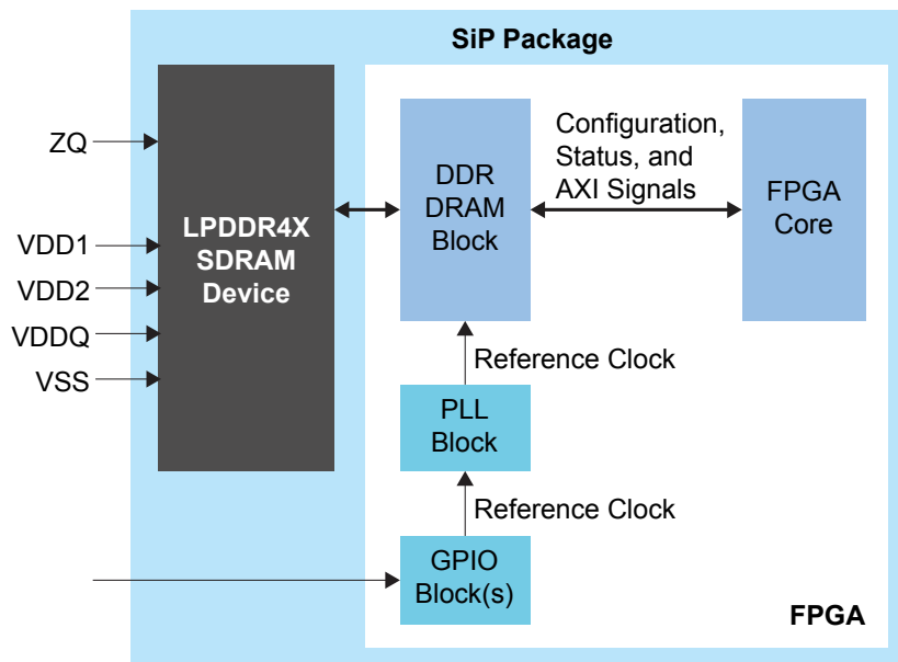
Figure 34: LPDDR4x SDRAM Interface Block Diagram
