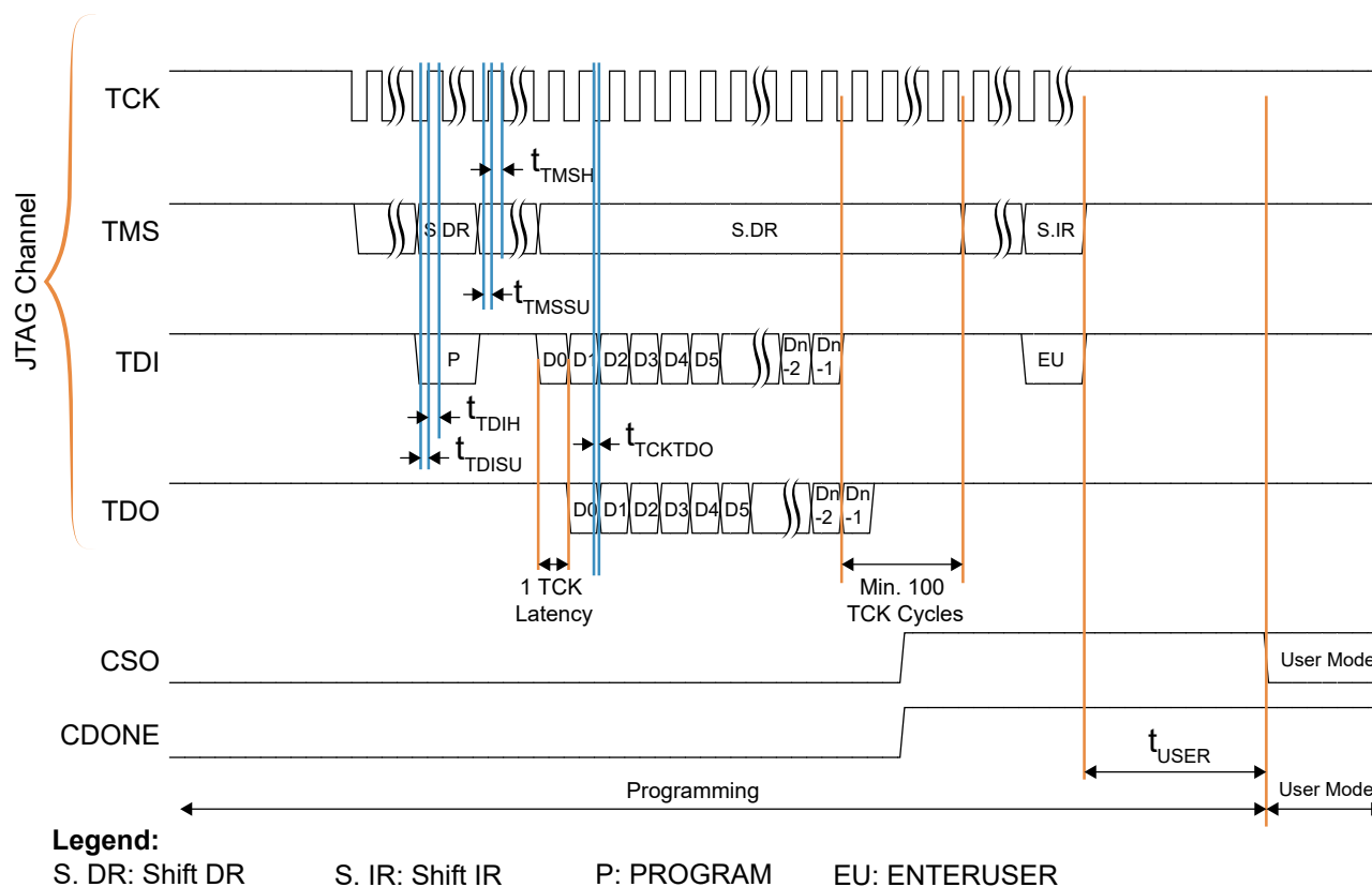
Figure 51: JTAG Timing Waveform
