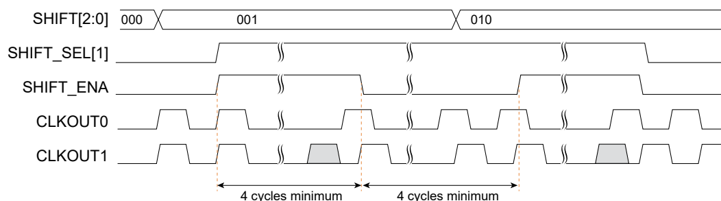
Figure 42: Consecutive Dynamic Phase Shift Waveform Example for CLKOUT1
