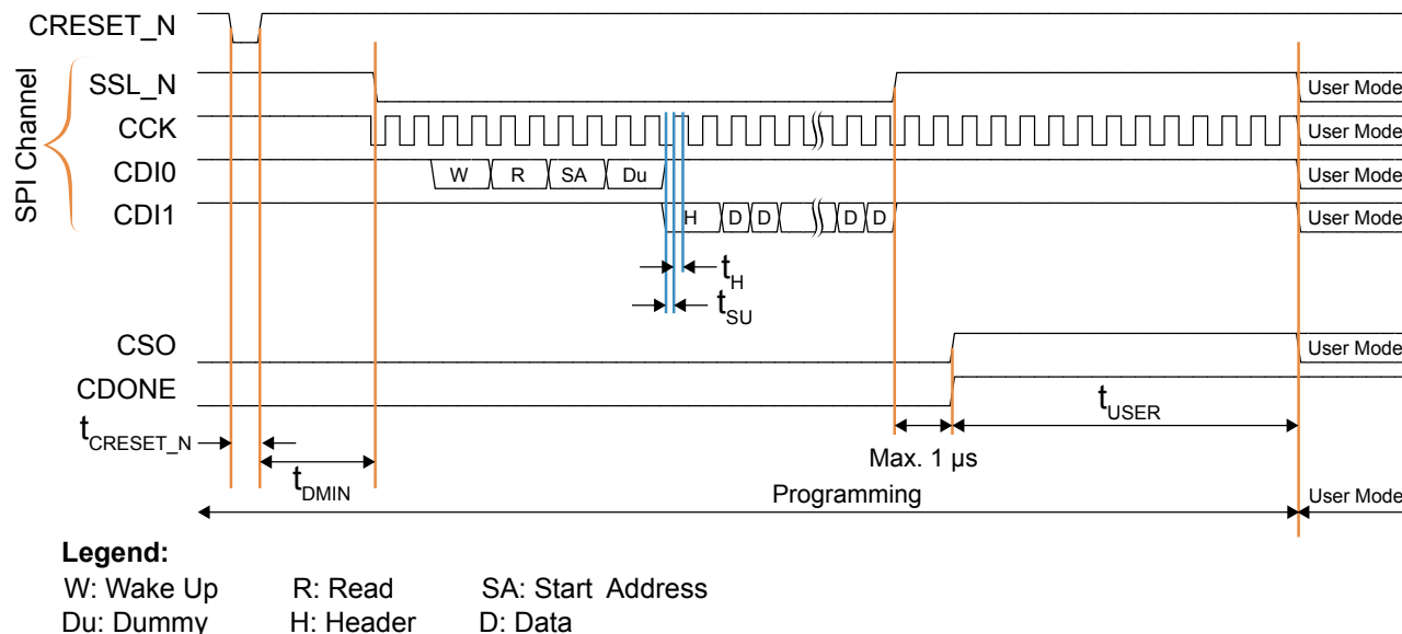
Figure 50: SPI Active (x1) Timing Sequence
