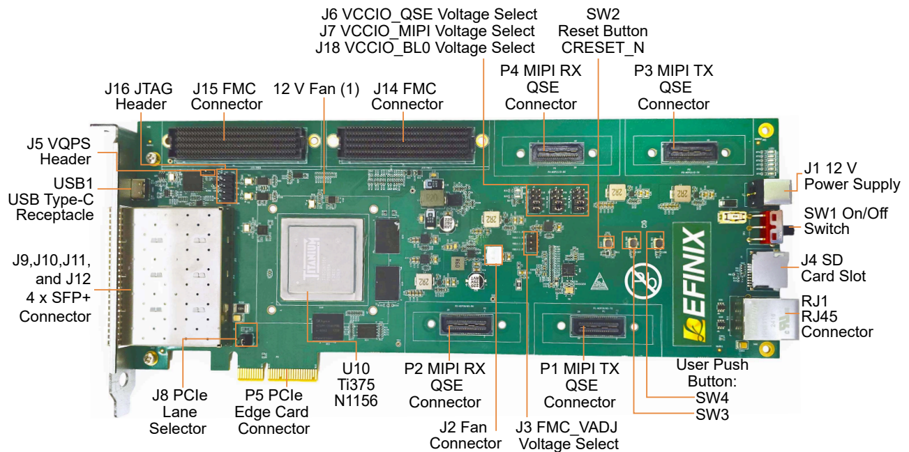
Figure 2: Titanium Ti375 N1156 Development Board Components
