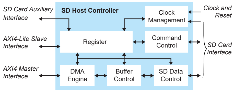
Figure 1: SD Host Controller PLL Calibration Block Diagram
