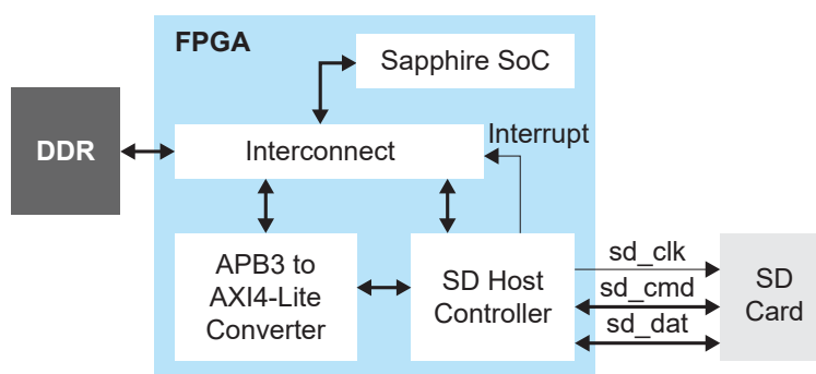
Figure 3: Standalone Example Design Block Diagram
