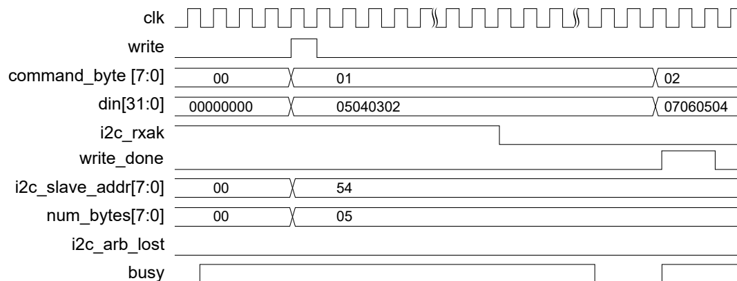
Figure 5: Multiple Write Operation on I 2 C Master Waveform
