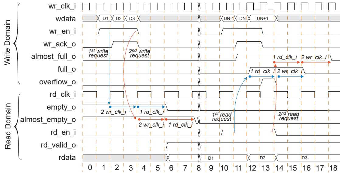
Figure 15: Asynchronous FIFO FWFT Mode Faster Write Clock with PIPELINE_REG=1
