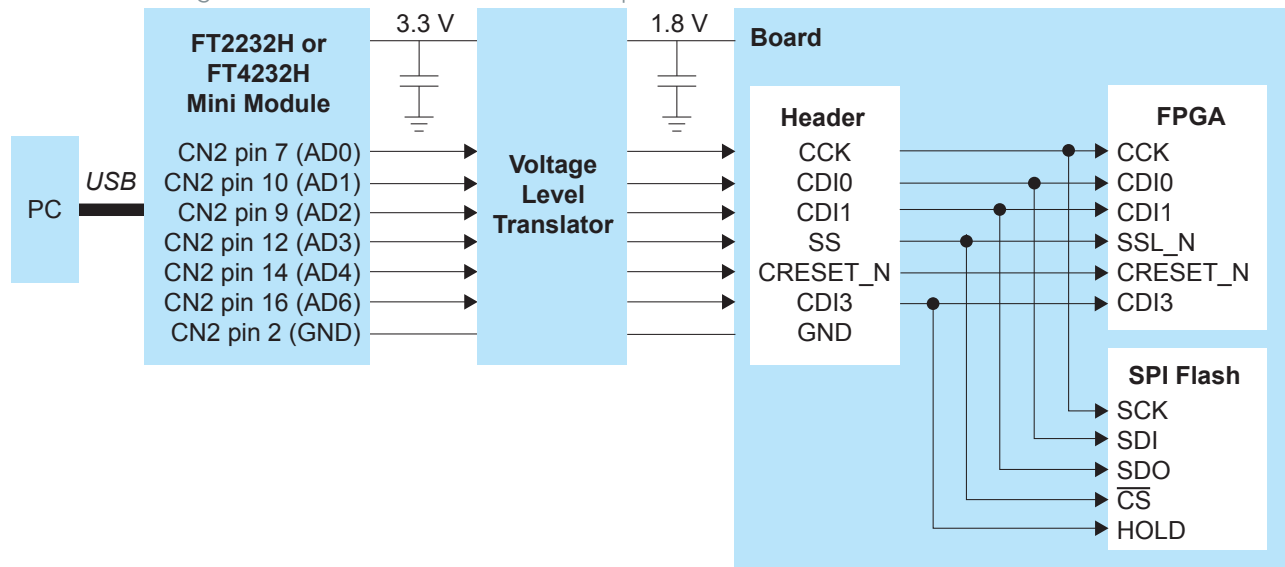
Figure 51: SPI Flash Programming with FTDI FT2232H and FT4232H Mini Module Connections (Titanium FPGAs)
