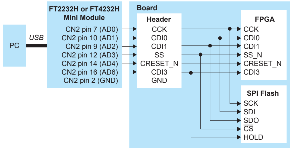
Figure 51: SPI Flash Programming with FTDI FT2232H and FT4232H Mini Module Connections (Titanium FPGAs)
