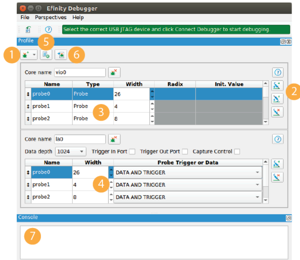
Figure 31: Debugger Profile Editor Perspective
