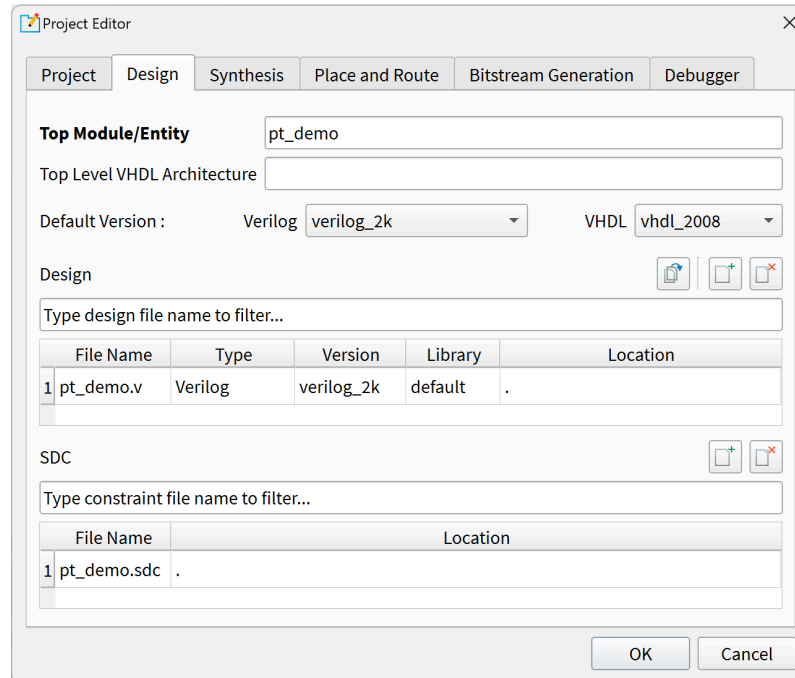
Figure 5: Project Editor - Design Tab
