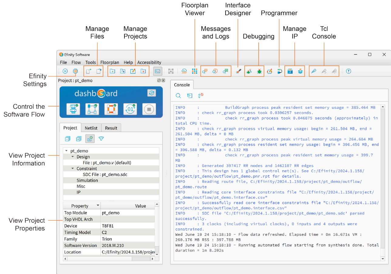
Figure 3: Efinity Main Window
