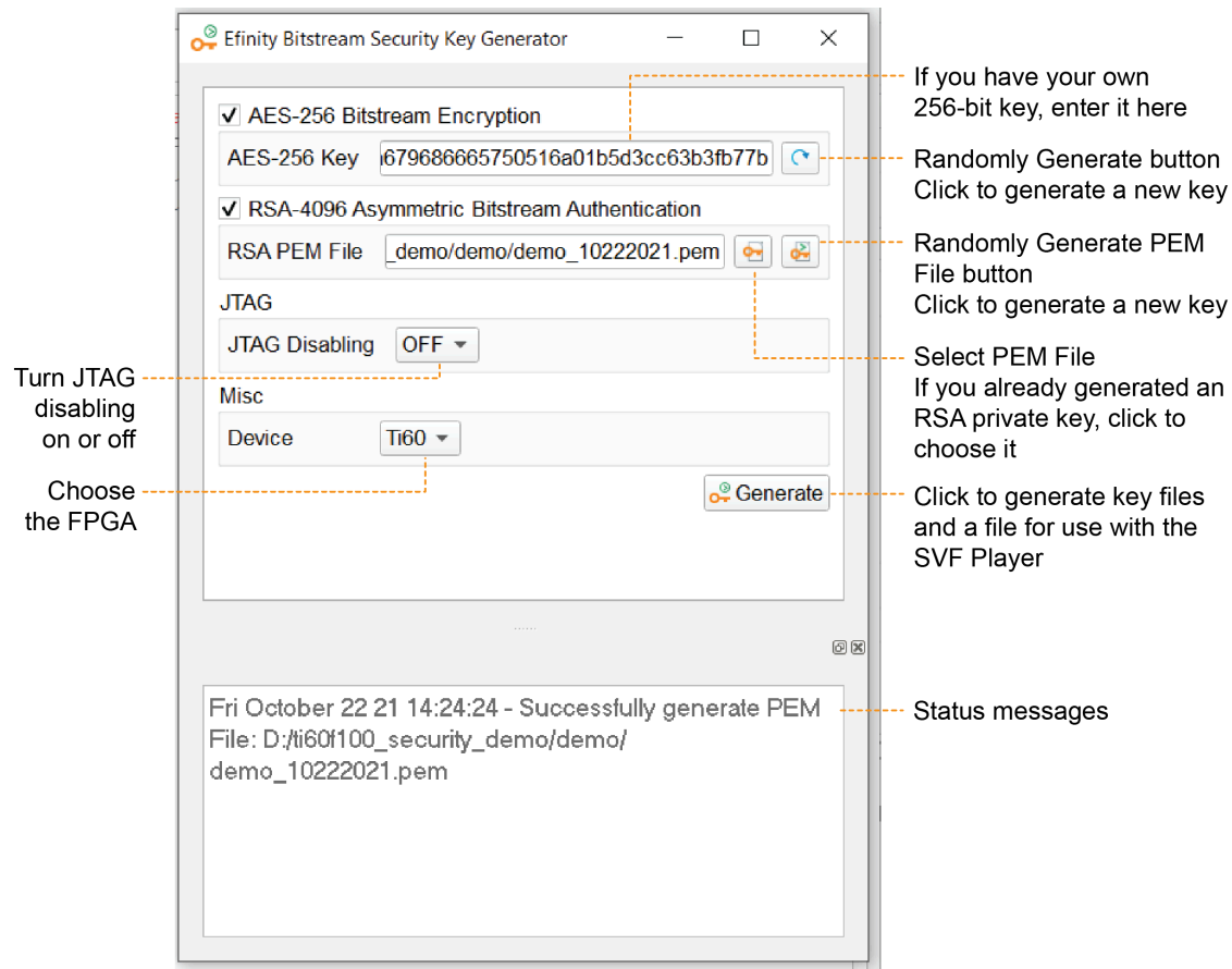
Figure 46: Efinity Bitstream Security Key Generator
