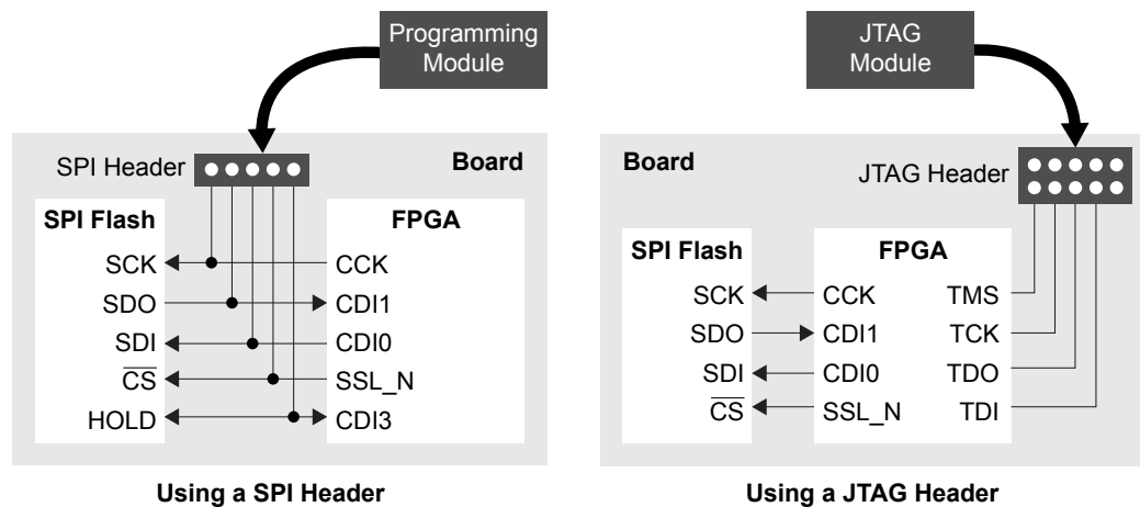
Figure 37: Flash Programming Board Setup
