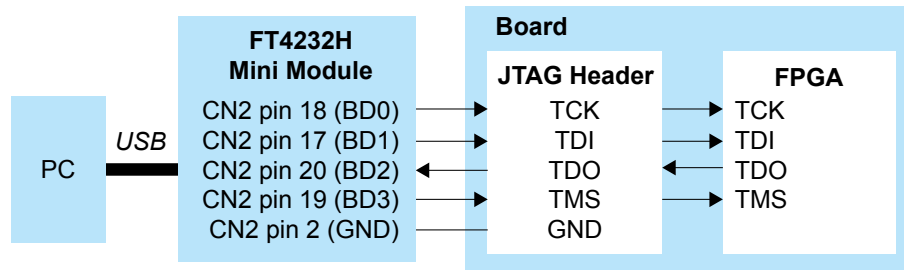
Figure 55: Connect FT4232 Mini-Module to JTAG Pins
