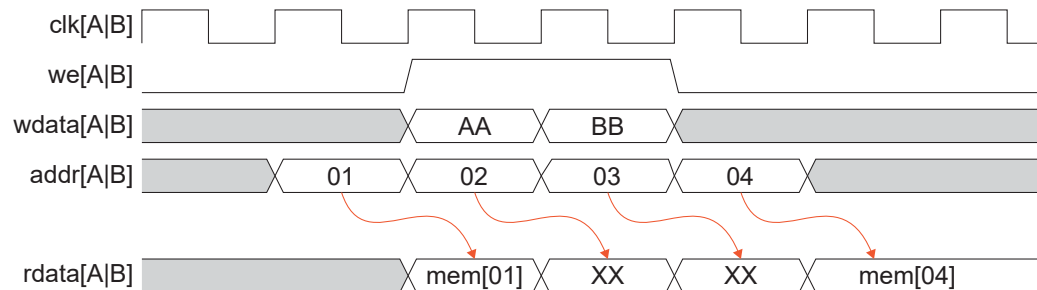
Figure 11: Read Unknown Mode Example (Single-Port and Simple Dual-Port RAM)
