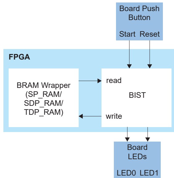
Figure 17: BRAM Wrapper Example Design Block Diagram
