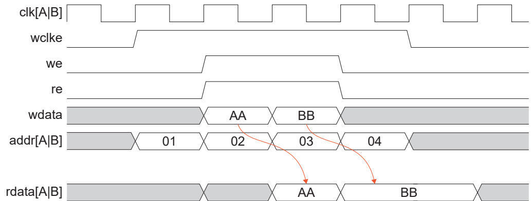
Figure 6: Write First Mode Example (Single-Port)
