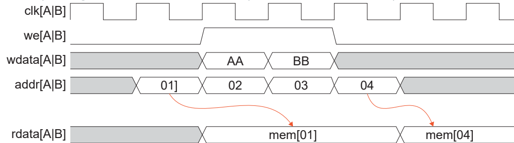
Figure 10: No Change Mode Example (True Dual-Port RAM)
